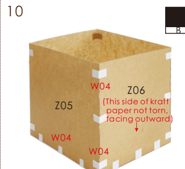
The junction of two pieces of plexiglass needs to be fixed with W04 (to prevent the plexiglass falling off)
