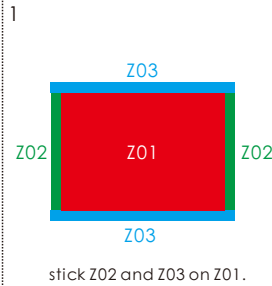
Ratio:1:10 Z03 plexiglass (transparent) 20*14.5*0.18(2pieces)
