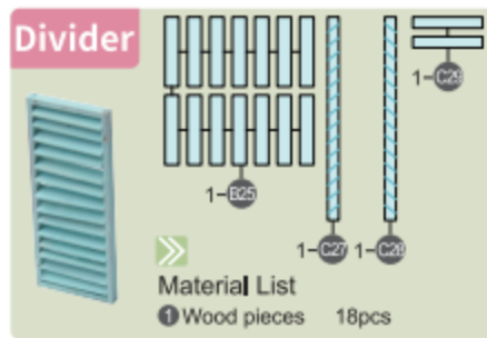
Glue as shown. (B25 is slightly tilted.)
