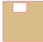
C03panel(white) 0.5X16.3X16(1pc)
